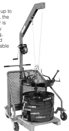
DP-1-23B Electric-powered DF-23 for power equipment only. Cover required for strap over 0.023" (0.58 mm). (Part No. 043584).
